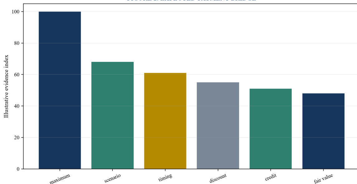
FIGURE 2. EXPECTED-PAYMENT BRIDGE
