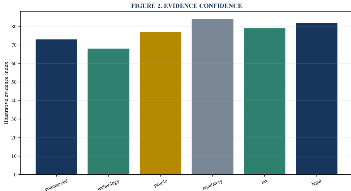
Figure 2. Evidence confidence
